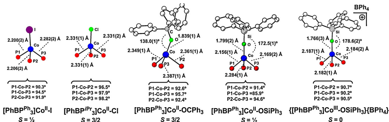
Fig. 4. Select structural data for a series of pseudotetrahedral [PhBP^R_3]Co-X species that feature both high- and low-spin ground-states.
