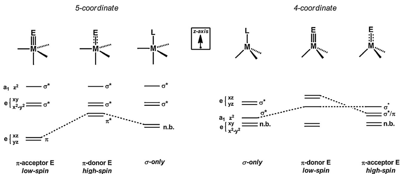
Fig. 7. Qualitative d-orbital splitting diagrams for 4- and 5-coordinate C_{3v} species, with the anticipated spin-state for each M(E) type noted.
