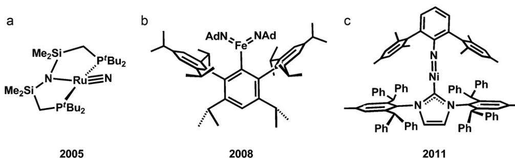
Fig. 8. Select examples of M(E) species with low coordination numbers. (a) [(^t\text{Bu}_2\text{PCH}_2\text{SiMe}_2)_2\text{N}]\text{Ru}^{\text{IV}}\text{N} [157], (b) (\text{Ar})\text{Fe}^{\text{V}}(\text{NAd})_2 [46], (c) (\text{IAr})\text{Ni}^{\text{II}}(\text{NAr}^*) [158].
