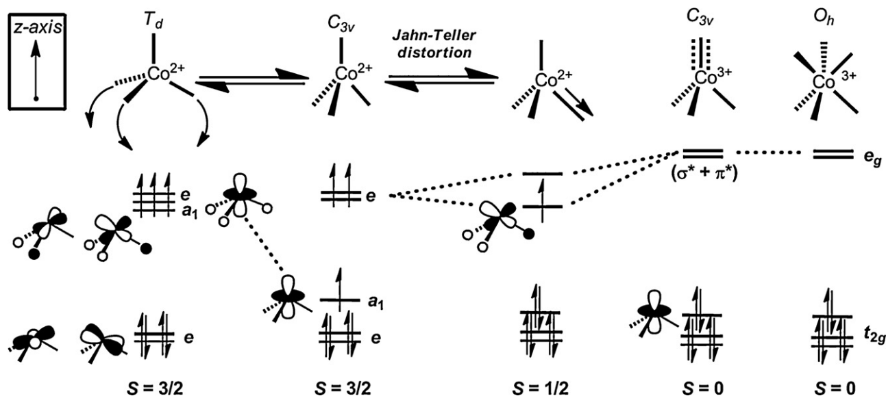
Fig. 3. Qualitative d-orbital correlation diagram that summarizes the electronic relationships discussed in the text regarding 4-coordinate L_3Co-X species.
