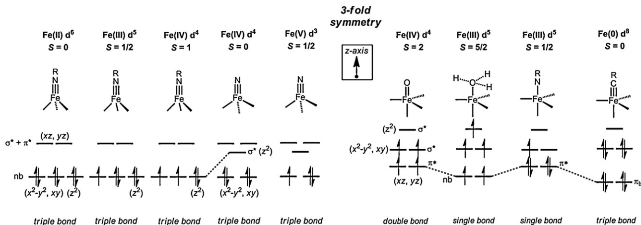
Fig. 2. Qualitative d-orbital splitting diagrams for L_3 - Fe(E) and L_3L - Fe(E) structure types discussed throughout the review. The diagram is meant as a guide to the discussion in the text. The relative ordering of the orbital energies for the lower-lying e set ( xy , x^2-y^2 ) and the a_1 orbital ( z^2 ) is not implied for L_3Fe(NR) structures, and are arbitrarily set as degenerate, for simplicity.
