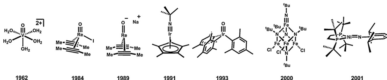
Fig. 1. Examples of M\equiv E and M=E species, with year of publication noted.
