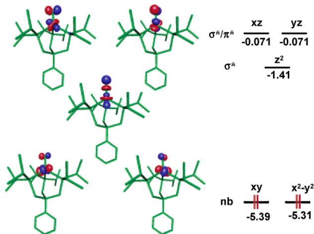
Fig. 6. Theoretically predicted geometry and electronic structure (DFT, JAGUAR 5.0, B3LYP/LACVP**) for S=0 [PhBP^{iPr}_3]Fe=N . Lobal representations correspond to the frontier orbitals (energies in eV). Structural parameters: Fe–P = 2.28, 2.28, 2.29 Å; N–P–Fe = 117, 117, 119°; P–Fe–P = 99, 101, 101°; Fe–N = 1.490 Å.
