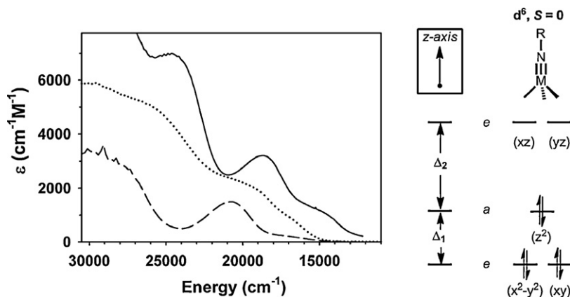
Fig. 5. (a) Visible absorption spectra of d^6 pseudotetrahedral metal imides. All spectra were recorded at room temperature. (A) [\text{PhBP}^{\text{Ph}_3}]\text{Co}(\text{NPh}) (—); (B) [\{\text{PhBP}^{\text{Ph}_3}\}\text{Fe}(\text{NAd})\}^- (···) in THF; and (C) [\text{PhBP}^{\text{Ph}_3}]\text{Co}(\text{N}^t\text{Bu}) (---). (b) d-orbital splitting diagram defining splittings \Delta_1 and \Delta_2 .
